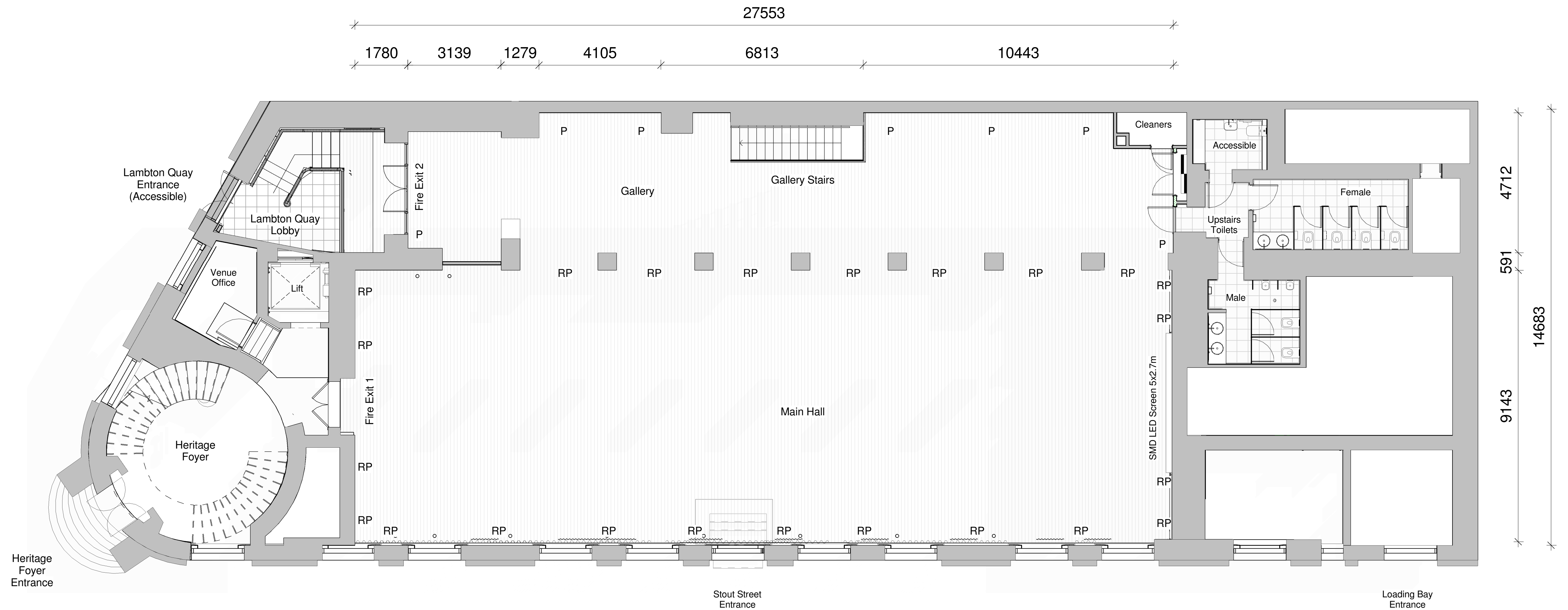
1 Ground Floor Layout 1 : 75
